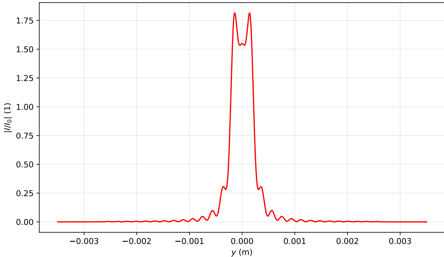
Intensity profile I(x=0, y, z=0.159)/I_0 , P_{in}=3.0P_{cr} , artificial time
